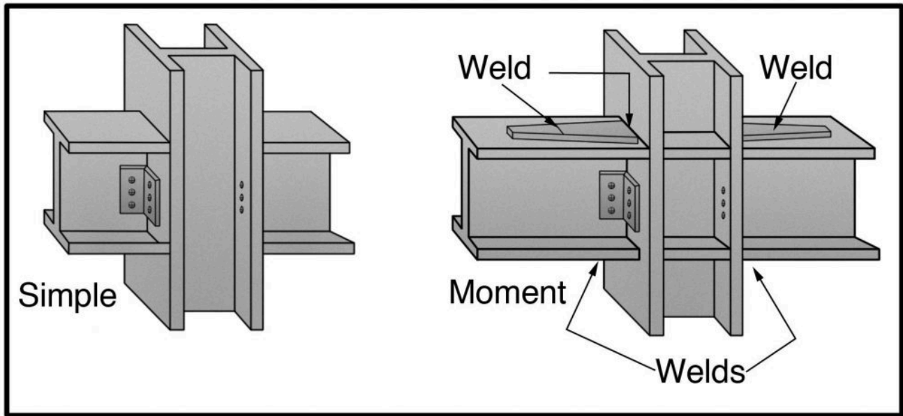
Figure 12-6. Joint used in a moment-resistant frame.
