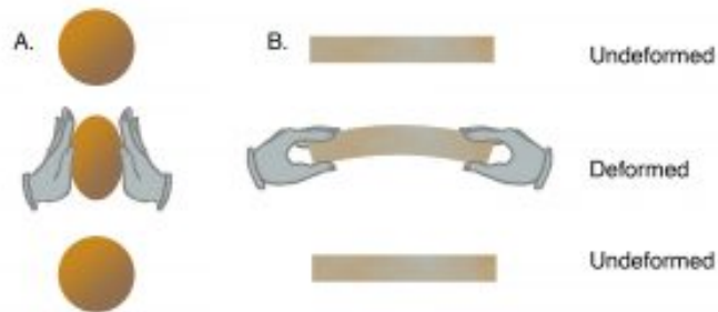
Figure 3-1. Elasticity. (a) An inflated balloon is squeezed between two hands, changing its shape. If the hands are removed, the balloon returns to its earlier shape. (b) A thin board is bent into a curved shape. If the hands bending the board are removed, the board returns to its original shape. The balloon and board are both elastic.
