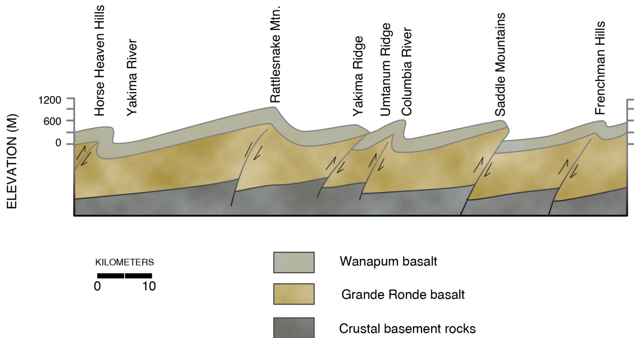
Figure 6-23. Geologic cross section across Yakima Fold Belt west of Hanford Reservation. Folds in basalt are interpreted as being forced up by compressional faults in rigid crust beneath the basalt; these faults may be earthquake sources. South is to the left.
