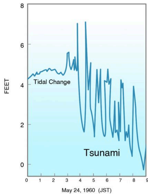
Figure 4-17. (Top) Wave fronts of tsunami accompanying the 1960 Chilean Earthquake (Mw 9.5) in hours, as tsunami crossed Pacific. (Bottom) Tide gauge record of 1960 tsunami recorded at Miyako, Japan, in hours. From K. Satake, University of Tokyo.
