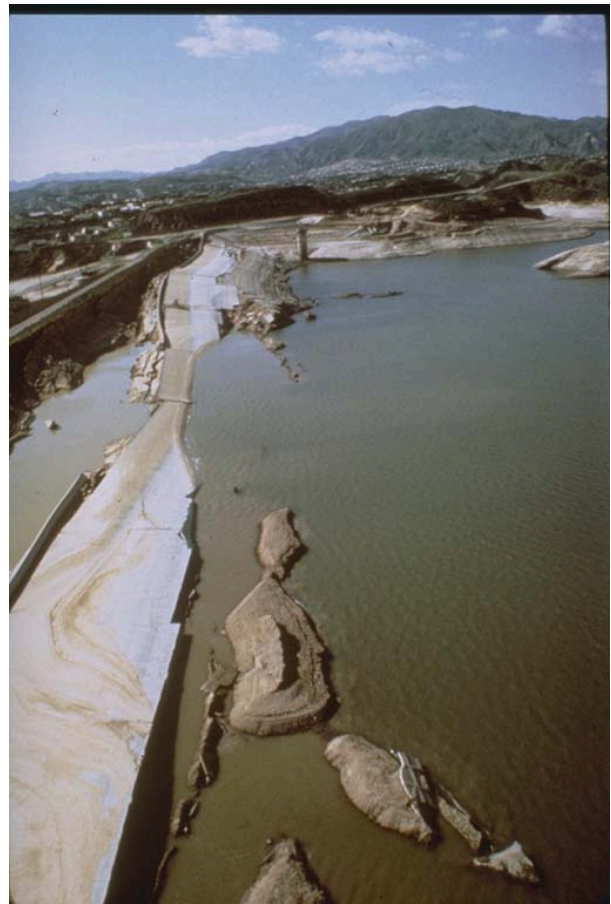
Figure 12-16. Van Norman Dam, San Fernando Valley, California, after the 1971 Sylmar Earthquake. About eight hundred thousand yards of the embankment, including the parapet wall, dam crest, most of the upstream slope, and a portion of the downstream slope, slid into the reservoir, causing a loss of about thirty feet of dam height. Fortunately, the dam was only about half full at the time. Eighty thousand people living downstream from the dam were ordered to evacuate, and steps were taken to lower the water level in the reservoir. Photo by E. V. Leyendecker, USGS
