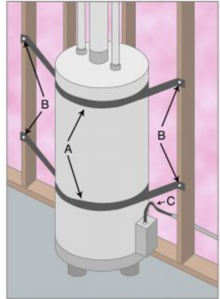
Figure 11-8. Strap water heater, top and bottom, with metal straps (A) which completely encircle the heater and are attached to studs (B). If the water is heated by gas, the gas supply line (C) should be flexible. In this example, water heater rests against stud. If water heater is against drywall or plaster wall, brace it with a two-by-four so that it does not bang against the wall.
