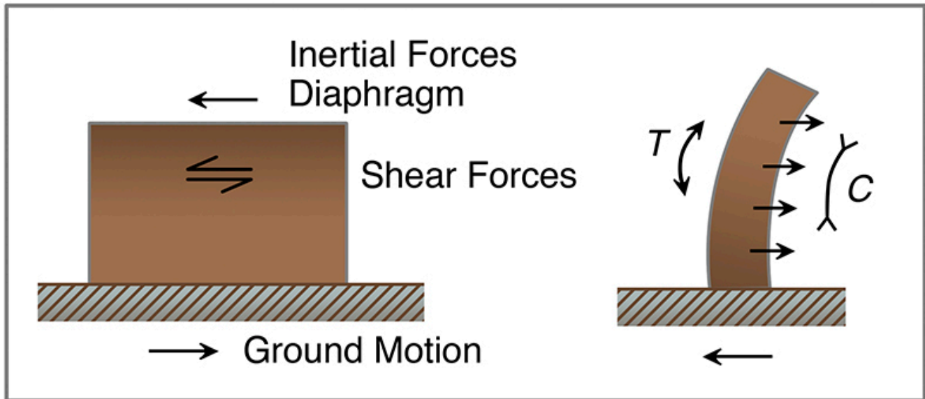
Figure 12-5. Shear walls resist shear stresses transmitted from the ground and bending stresses in slender, tall buildings. C, compression; T, tension. From AIA/ACSA Council on Architectural Research.
