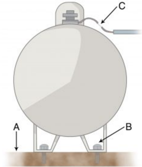
Figure 11-15. Propane tank. Mount tank on six-inch-thick concrete pad (A) using four half-inch diameter bolts (B) with three-inch minimum embedded into concrete. Provide a flexible hose connection (C) between tank and the rigid supply line. From Humboldt State University
