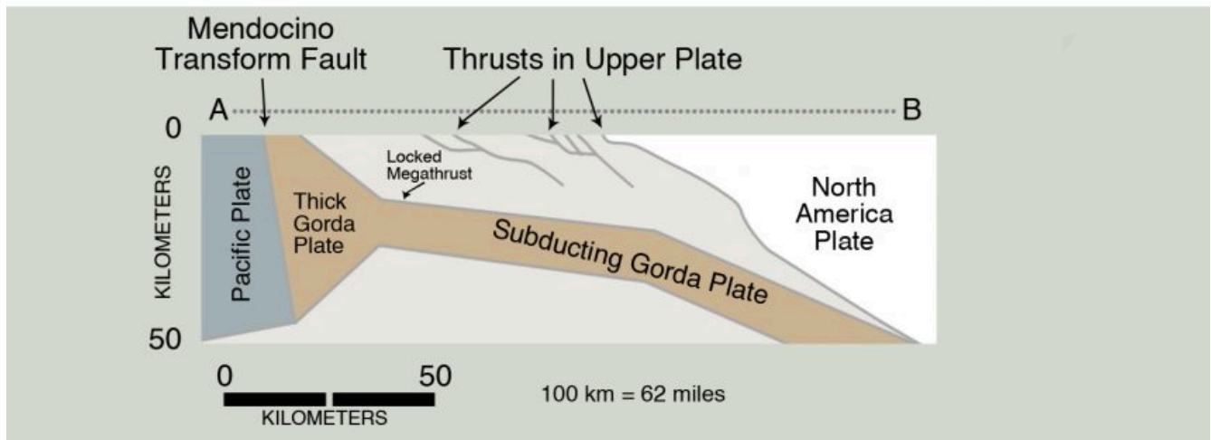
Figure 5-2. The Cascadia Subduction Zone approaches the coastline in northern California, where active folds and thrust faults have been studied by Gary Carver and his associates at Humboldt State University. The subduction zone ends at the Mendocino Transform Fault, which turns southeast to become the San Andreas Fault. The Gorda Plate and spreading center (Gorda Rise) are also shown. The plate is being internally deformed along the Cascadia Subduction Zone and Mendocino Transform Fault.
