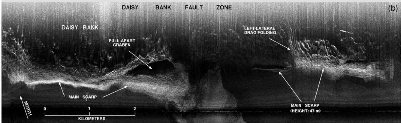
Figure 4-3a. Sidescan sonar image of Daisy Bank strike-slip fault west of Newport. These structures are similar to those on subaerial faults in California. Image from Chris Goldfinger.
