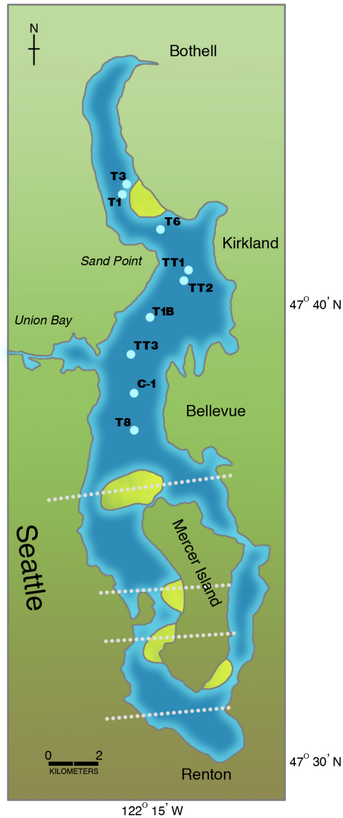
Figure 6-2. Map of Lake Washington, bordering the city of Seattle on the east, locating major landslides and sunken forests (coarse dot pattern). Dashed lines extending across southern half of lake are possible traces of the Seattle Fault. Solid circles are piston core sites that are correlated in Figure 6-5. Modified from Robert Karlin, University of Nevada Reno, and Sally Abella, University of Washington
