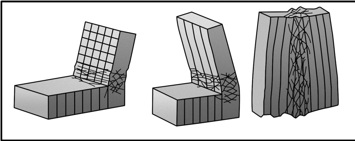
Figure 12-13. Buildings have a vibrational frequency depending on their height. If the vibrational frequency resonates with that of the earthquake waves, shaking will be amplified, and damage will be more severe, as was the case in Mexico City in the 1985 earthquake. From Bolt (2004)
