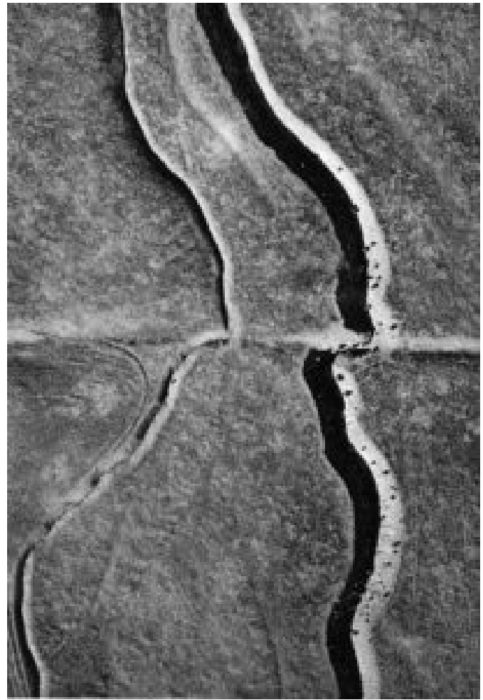
Figure 3-5b. Right-lateral strike-slip fault. Offset furrows in a cultivated field near El Centro, California, during an earthquake on October 15, 1979.
