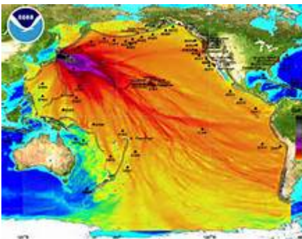
Figure 9-14. Tsunami wave heights from the Tohoku-oki earthquake of March 11, 2011. Darker colors indicate higher wave heights. Note location of DART buoys. Source: NOAA.
