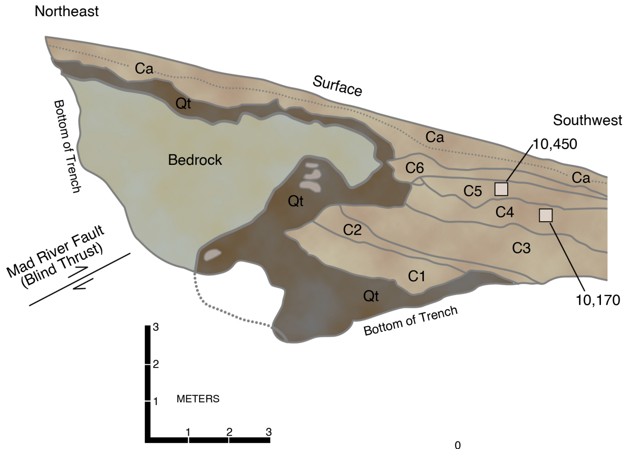
Figure 6-36. Log of side of backhoe trench across a scarp of the Mad River Thrust Fault at McKinleyville, California, showing how bedrock has been thrust over sediments that are radiocarbon dated at about ten thousand years. Laboratory errors are \pm 60 -80 years. The bedrock is overlain by a wave-cut platform which is itself overlain by terrace deposits (Qt). These were folded, indicating that the Mad River Fault is a blind thrust at this locality. The terrace deposits are overlain by debris from the rising fault scarp (C1 through C6); each unit may have been deposited during an earthquake. Ca marks the active slope wash and debris. Modified from a sketch by Gary Carver, Humboldt State University
