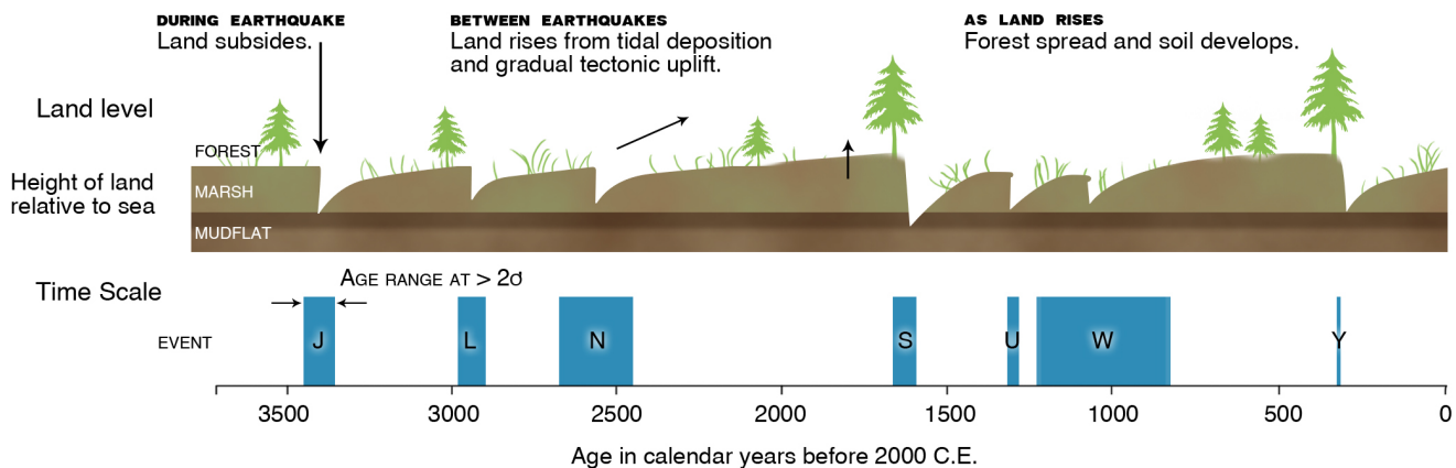
Figure 4-21. Evidence for earthquakes at Redtail locality at Willapa Bay, Washington. Horizontal line is time in years; vertical line is elevation with respect to sea level divided into coastal forest, marsh, and tidal mudflats. Heavy line shows change in elevation. Ground sinks abruptly to sea level after an earthquake, then gradually rises to a marsh environment or a forest environment. Letters identify earthquakes dated by radiocarbon, with the gray band representing uncertainty in dating. The youngest, event Y, is the earthquake of A.D. 1700, dated by tree rings and a tsunami in Japan. The time interval between earthquakes varies from nearly one thousand years between events N and S to less than three hundred years between events U and W. The longest interseismic intervals allowed the ground to develop forests before they were drowned by earthquakes S and Y, whereas earthquakes N, U, and W struck when the ground had only risen to develop a coastal marsh. The greater vertical drop for earthquakes J, S, and Y suggests that they may have been larger than earthquakes N, U, and W. After B. Atwater and E. Hemphill-Haley, USGS
