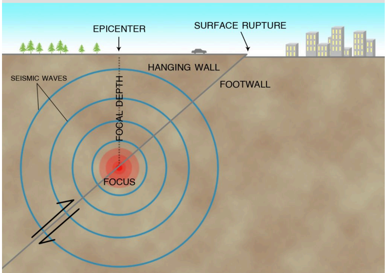
Figure 3-4. A cross section of the Earth's crust.
