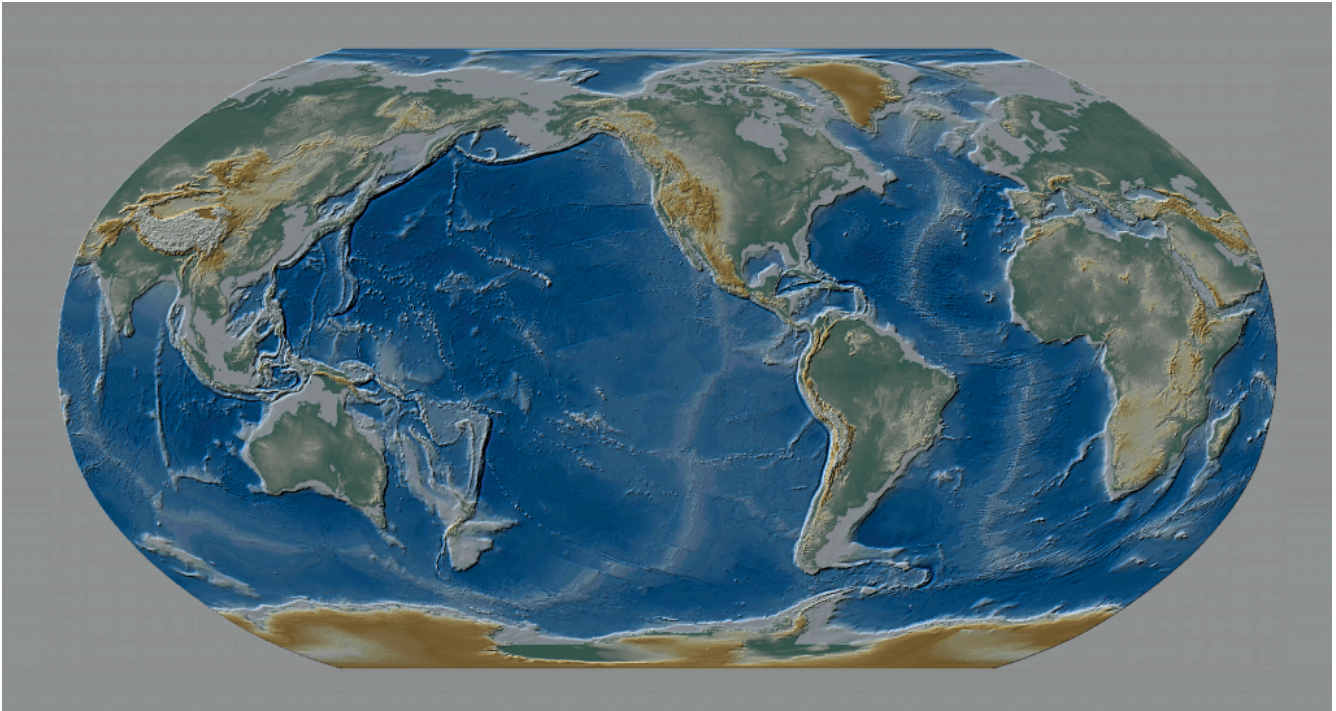
Figure 2-3a. World map with oceans removed. Ocean floor in shades of blue; lightest bands show oceanic spreading centers (Mid-Atlantic Ridge, East Pacific Rise) and very dark bands show trenches, the boundaries of subduction zones. Light band at west edge of North America locates continental slope, at base of which is Cascadia Subduction Zone.
