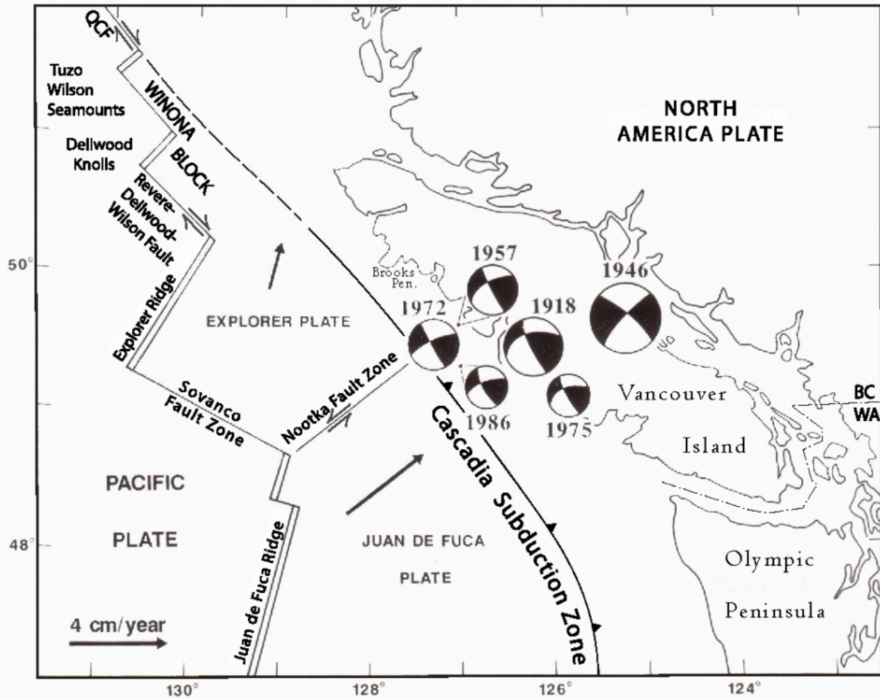
Figure 6-19. Earthquakes northeast of Nootka fault zone and central Vancouver Island. The Nootka fault zone separates the Juan de Fuca and Explorer plates. The beach-ball plots show that all earthquakes were due to left-lateral strike slip; larger earthquakes have larger beach balls. The 1918 and 1946 earthquakes were in North American continental crust. The 1946 earthquake was the largest recorded crustal earthquake in the Cascadia region. QCF: Queen Charlotte fault.
