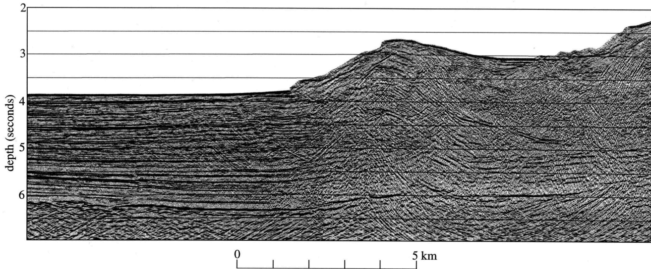
Figure 4-2. Seismic-reflection profile of the Cascadia Subduction Zone off central Oregon. West is to the left. Signals from a ship were bounced off the sea floor and off more deeply buried sediment layers, then echoed back to the ship, allowing a profile to be made that shows the geology beneath the sea floor. The flat sea floor on the left is the sediment-covered abyssal plain of the Juan de Fuca Plate. The Cascadia Subduction Zone has thrust highly deformed rocks of the North America Plate over the flat Juan de Fuca Plate. The fault slopes gently to the east. Sediment layers at the left are being forced under the edge of the continent and, in addition, dragged up against the edge of the continent as an accretionary wedge. Profile acquired in 1989 by Digicon for the National Science Foundation. Image courtesy of LaVerne D. Kulm and Chris Goldfinger, College of Earth, Ocean, and Atmospheric Sciences, Oregon State University.
