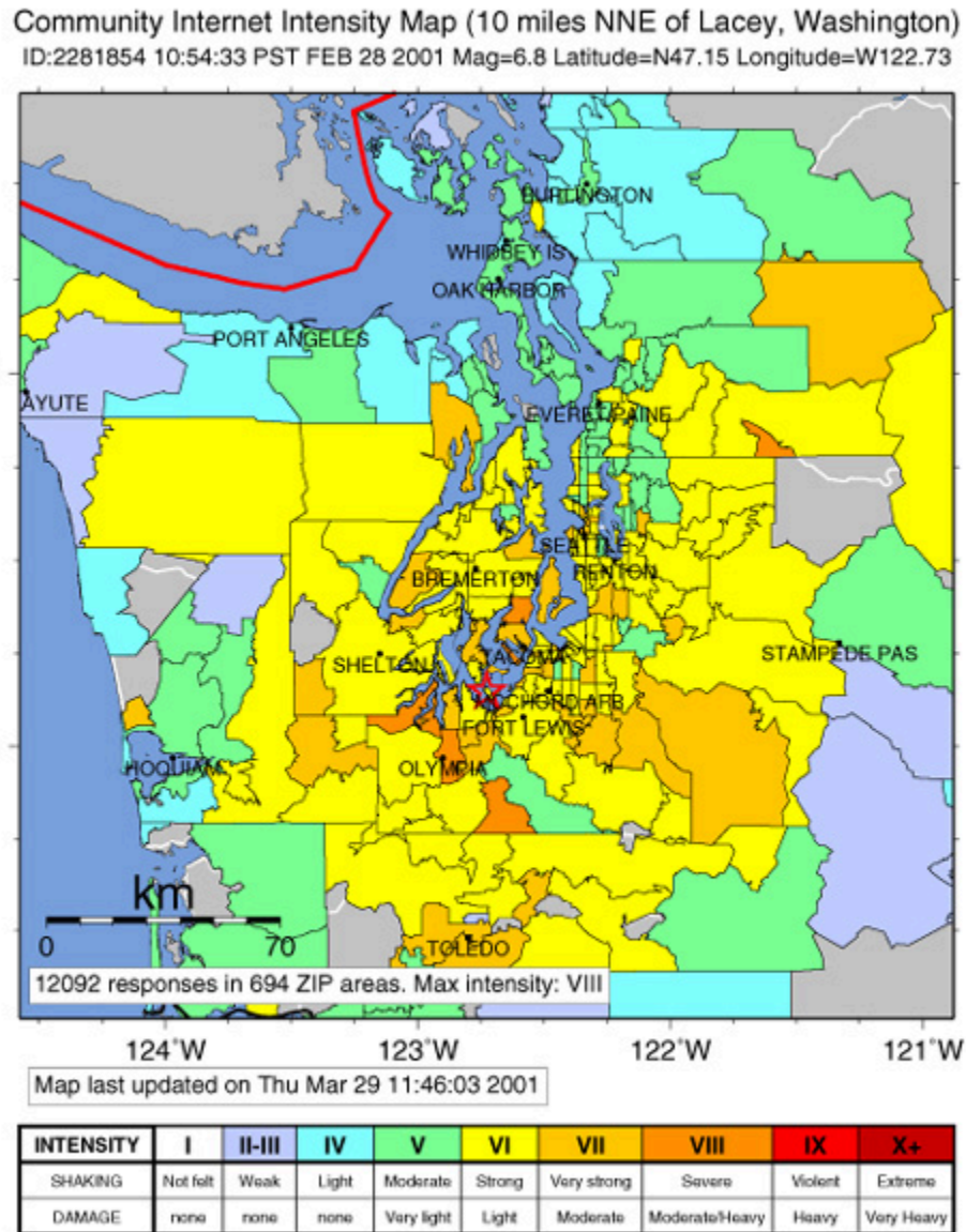
Figure 3-16. Community Internet Intensity map (CIIM) for the 2001 Nisqually Earthquake. Epicenter is the white star. Go to https://earthquake.usgs.gov/data/dyfi/ on the USGS Web site or to the PNSN website, which brings up “Did You Feel It?” along with a brief questionnaire. Log on and complete the questionnaire, which includes your ZIP code. The figure shows the result of 12,092 responses from 694 ZIP code areas. The lightest shading is intensity VI; darker shade close to epicenter is intensity VII and VIII. From USGS Fact Sheet 030-01.
