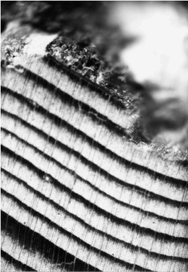
Figure 6-4 Tree rings from a 1,100-year-old tree dredged from the bottom of Lake Washington. Dark zone at top is the bark. Each pair of light and dark rings represents annual growth of one year. Photo by Gordon Jacoby, Columbia University
