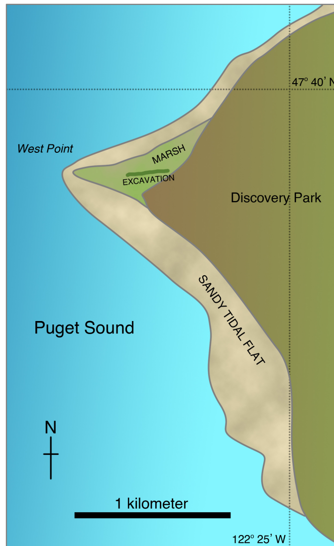
Figure 6-6. (a) Map of West Point area of Magnolia Bluff, Seattle, locating excavation depicted in Figure 6-6b (heavy line). Sandy tidal flat exposed only at very low tide. Discovery Park is an upland underlain by Pleistocene deposits. (1 km = 0.62 miles)
