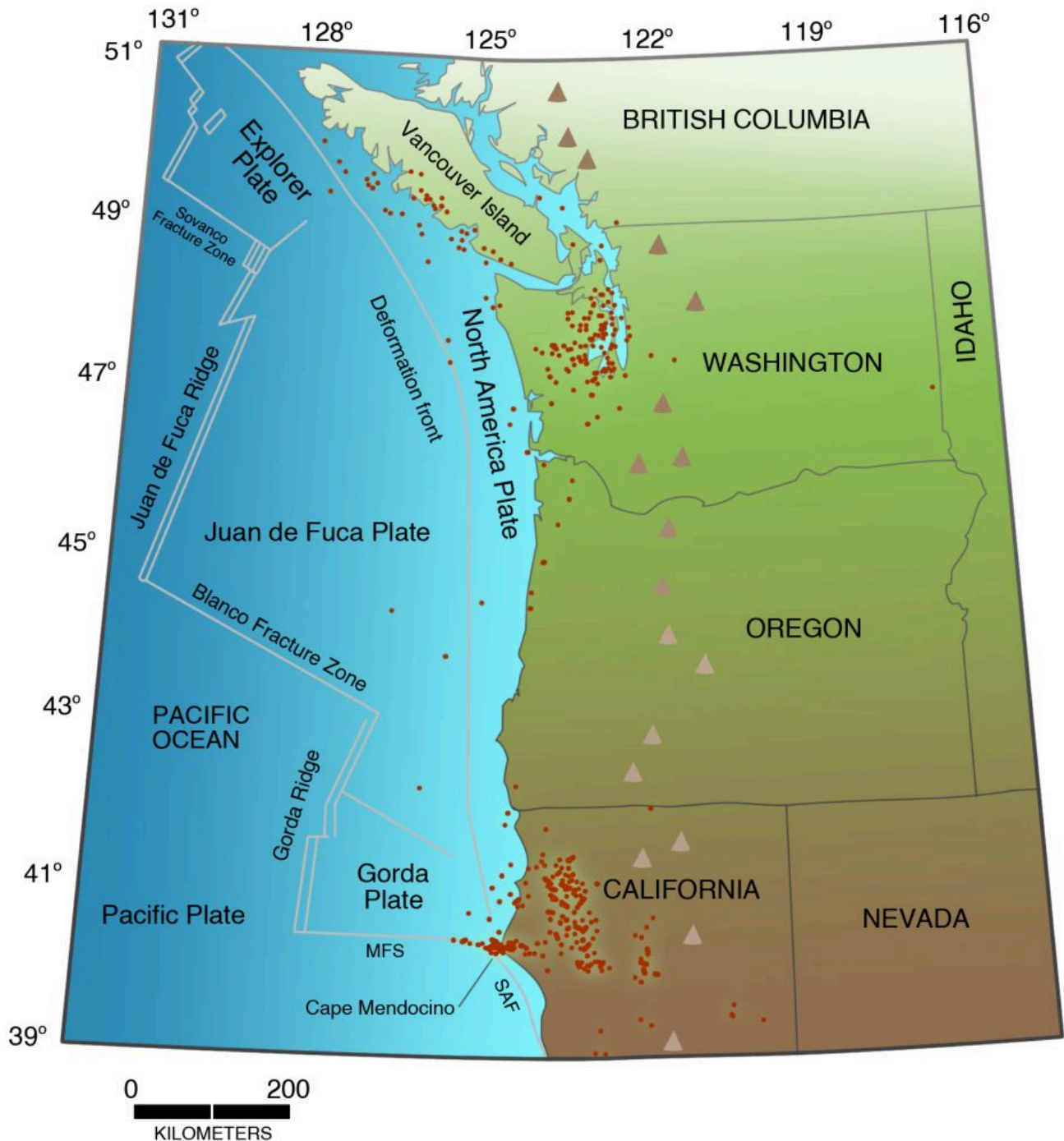
Figure 5-1. Distribution of earthquakes deeper than 16 miles in the Pacific Northwest. Most are intraplate earthquakes in the downgoing Juan de Fuca Plate. Earthquakes are not distributed evenly but are concentrated in Puget Sound, coastal Vancouver Island, and northwestern California. MFS, Mendocino Fracture System; SAF, San Andreas Fault; Heavy curved line in western Washington locates the top of the subduction zone at 60 km depth. Triangles: Cascade volcanoes. (100 km = 62 miles). From USGS Professional Paper 1560.
