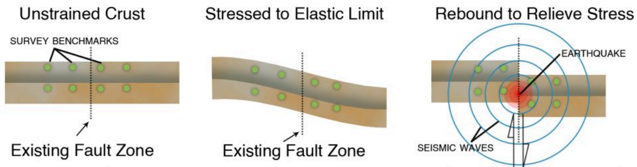
Figure 3-3. Illustration of elastic rebound theory of Harry F. Reid. Strain is building up.
