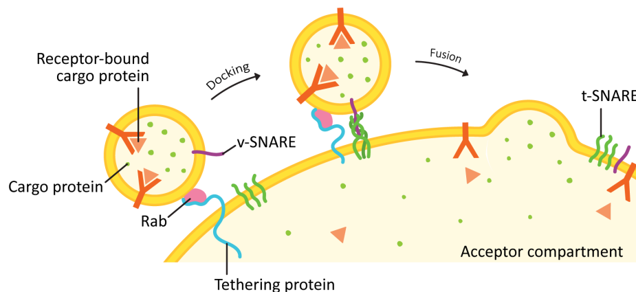
Figure 04-21: Docking and fusion. Tethers bind to Rabs to help bring the vesicle close to the target membrane (docking). When close enough, SNARE proteins interact to fuse the membranes together. This image was created by Heather Ng-Cornish and is shared under a CC BY-SA 4.0 license.
