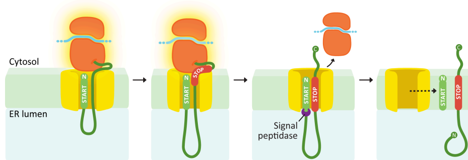
Figure 04-10: Insertion of a protein with an N-terminal START and a STOP insertion sequence.
