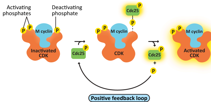
Figure 08-08: Positive feedback loop of Cdc25. Active M-CDK helps activate Cdc25, and this activation helps activate more M-CDK. This image was created by Heather Ng-Cornish and is shared under a CC BY-SA 4.0 license.
