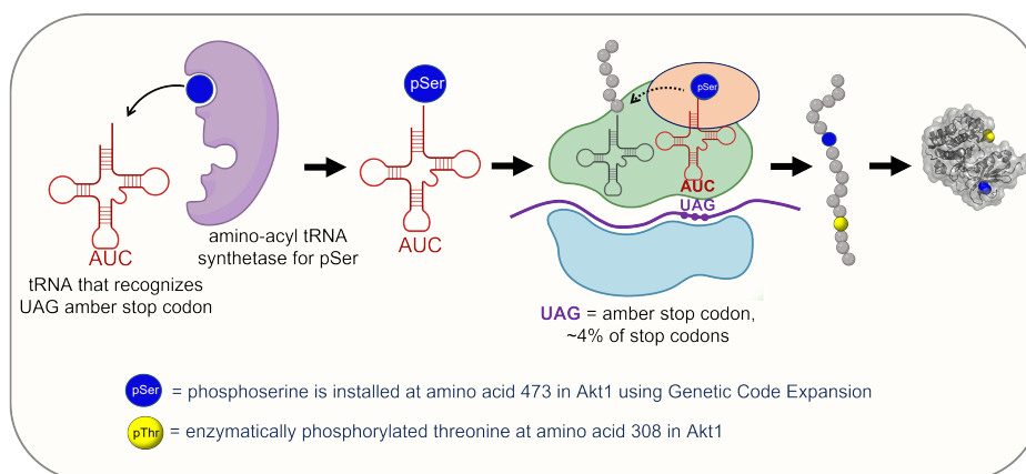
Figure 07-20: Schematic of genetic code expansion through the repurposing of a stop codon (UAG) so that it now codes for phosphoserine (pSer). To achieve this, an amino-acyl tRNA synthetase was genetically modified so that it could add a pSer to the UAG tRNA. Once this system is complete, genes can be modified to include UAG at a site where a pSer is desired, and it will be translated that way. This schematic was made by Dr. Richard Cooley and Dr. Kari van Zee in the GCE4All Research Center at Oregon State University and is shared under a CC BY-SA 4.0 license.
